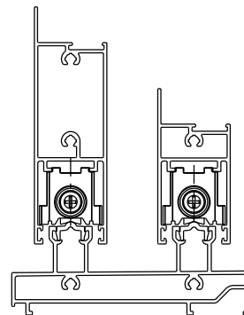
NOVA GOLD
