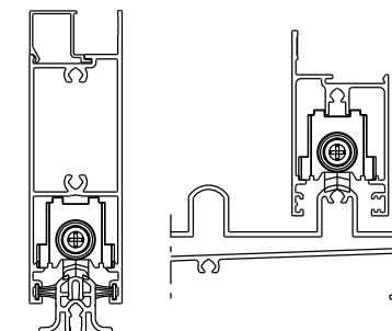
IMPERIAL 3.5 (porta/janela)
