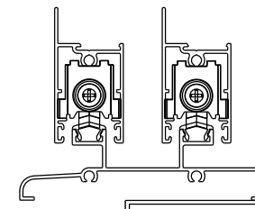
PRIME 32
