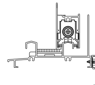
PERFILEVE 32
